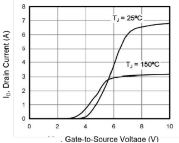
Figure 5. Transfer Characteristics
